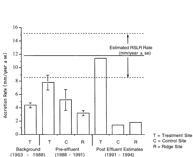
Figure 4. Background, pre-effluent, and post-effluent accretion rates (mean ± SE), relative sea-level-rise rates, and accretion balance deficits in the Pointe au Chene swamp.
