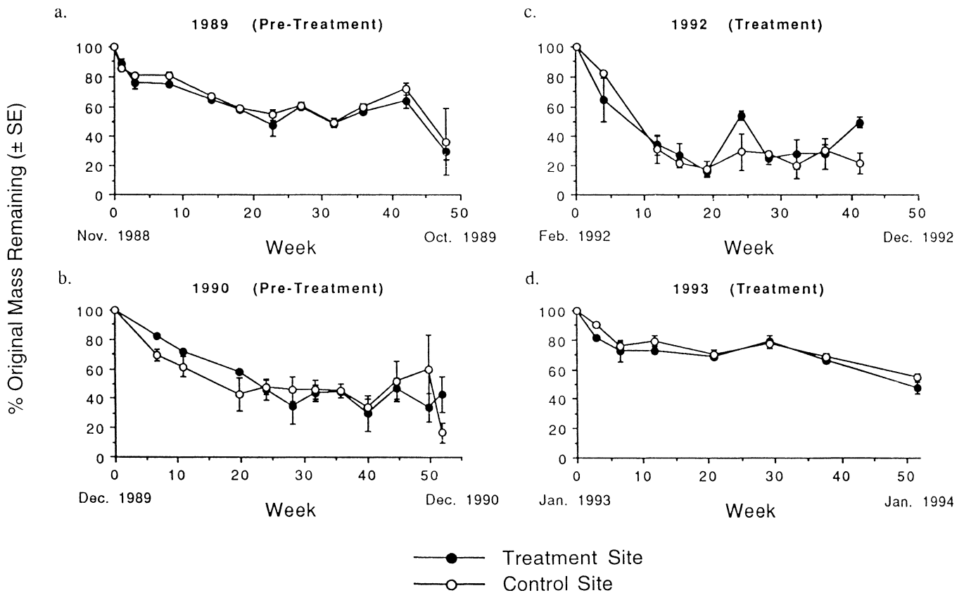
Figure 2. Percent of original dry mass remaining through time in the two Pointe au Chene sites during two pre-effluent years [1989 (a) and 1990 (b)] and two post-effluent years [1992 (c) and 1993 (d)].
