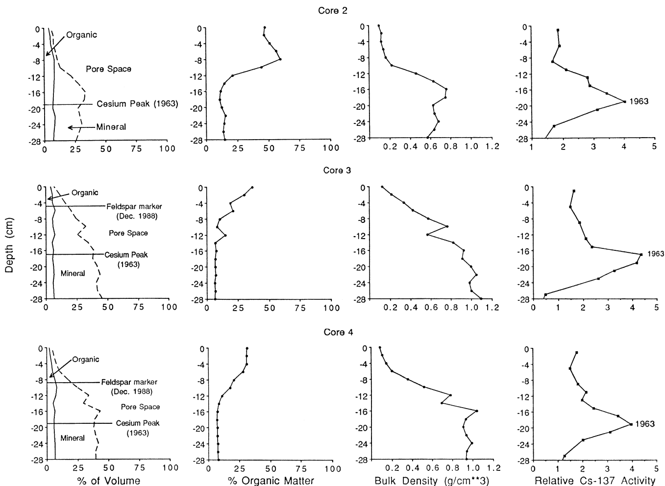
Figure 3. Volume distributions, percent organic matter (by weight), bulk density, and relative 137 Cs activity with depth in cores taken from the treatment site in October 1993. Cores 3 and 4 also contained a feldspar layer that marked the surface in December 1988.
