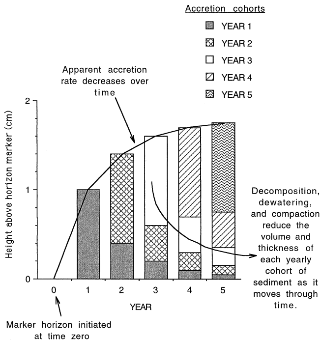
Figure 5. Conceptual diagram of sediment accretion dynamics above a horizon marker over time. Given that the yearly cohort of sediment is constant, the apparent rate of accretion (solid line) decreases with time because of decomposition and compaction.
